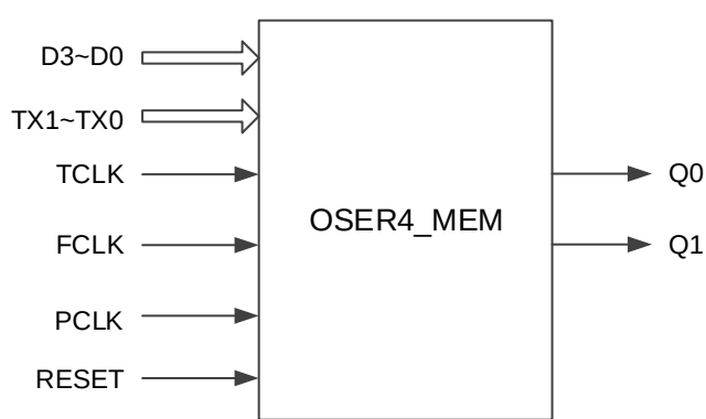
Figure 4-41 OSER4_MEM Diagram
