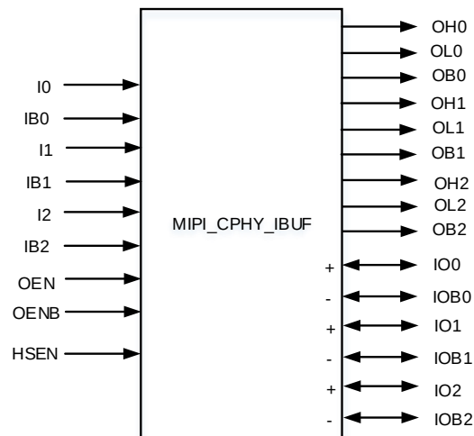
Figure 3-15 MIPI_CPHY_IBUF Port Diagram
