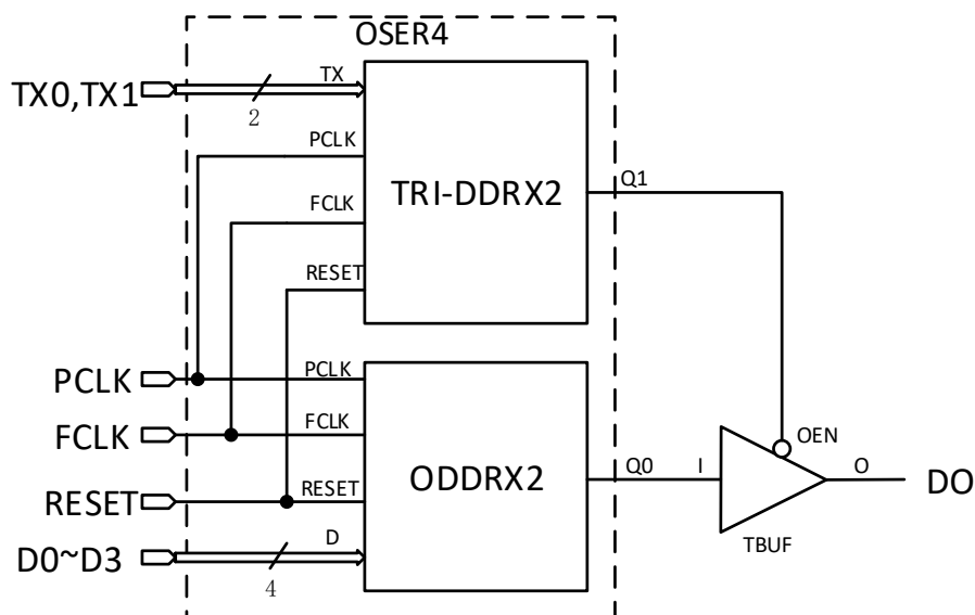
Figure 4-31 OSER4 Logic Diagram
