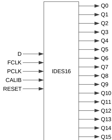
Figure 4-18 IDES16 Port Diagram
