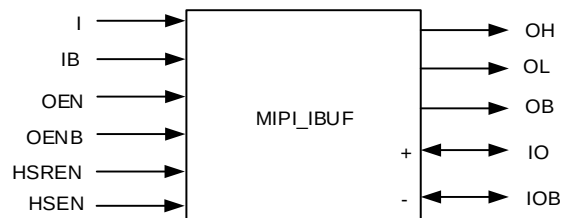
Figure 3-13 MIPI_IBUF Port Diagram
