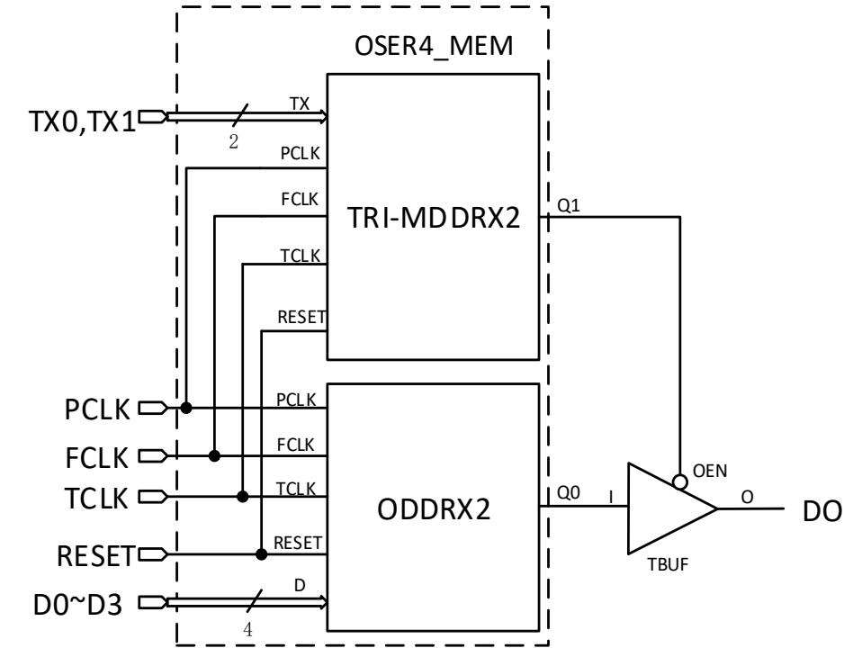
Figure 4-40 OSER4_MEM Logic Diagram
