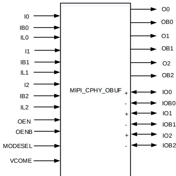
Figure 3-16 MIPI_CPHY_OBUF Port Diagram
