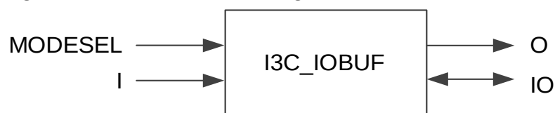
Figure 3-17 I3C_IOBUF Port Diagram
