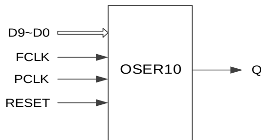
Figure 4-35 OSER10 Port Diagram
