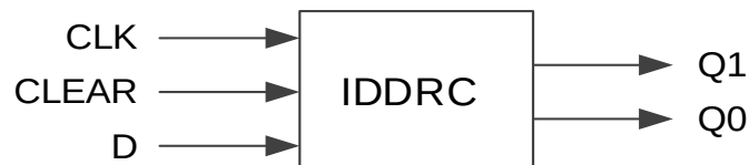
Figure 4-12 IDDRC Port Diagram
